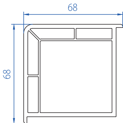
90° Corner Coupling 2108-3101
