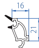
Casement Glazing Bead (24mm) 2107-4106
