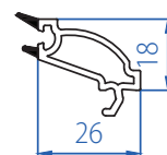
Sliding Glazing Bead (5-6mm) 3107-4101
