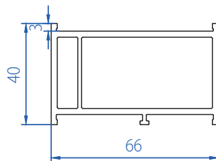
Coupling/ Extension Profile 2108-3106
