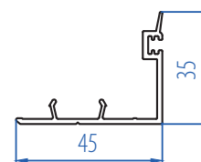
Sliding Window Interlock 2106-3101
