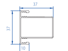
Super Screen Sash Mullion-3T 50502-11077
