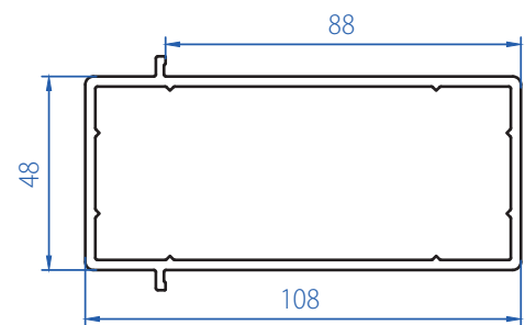
Large Coupling Profile 6108-3101
