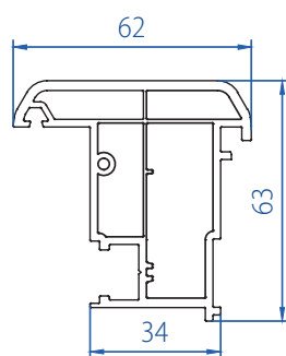
French Mullion 2102-1103
