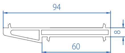
Casement-Sliding Profile Coupler (PRIMA) 50502-11039
