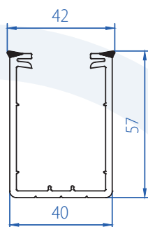
Stiffener Profile 2108-4107
