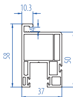
Fly Mesh Sash (For 3 Track) 2105-3106
