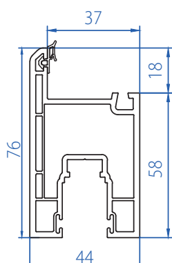
Sliding Sash 3105-1102
