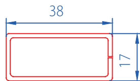
Mullion Reinforcement 1.5mm:9302-1504
