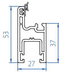
Eco Sliding Sash 4105-1101
