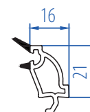
Casement Glazing Bead (For Sliding 10-12mm) 2107-4106
