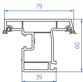
Outward Window Sash 2103-1101
