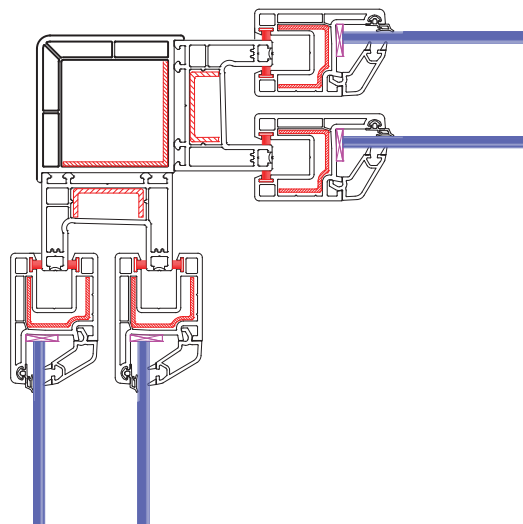
90° Corner Coupling 2108-3101
