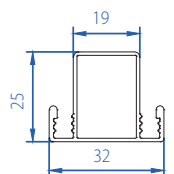
Fly Mesh Sash (Big) Mullion 50502-11058
