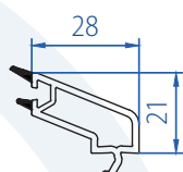
Casement Glazing Bead (12mm) 2107-4104
