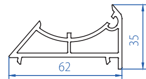
Bay Pole Adaptor 2108-3104
