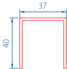
Mega Sash Reinforcement 2mm:9305-2003
