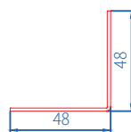
90° Corner Coupling 1.0mm:9208-1001
