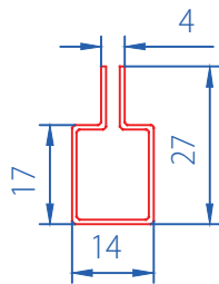
Sash/ Mullion 1.5mm :9502-1501
