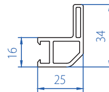
Clip On Frame 4104-3102
