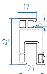
Fly Mesh Sash (Small) 2105-3104
