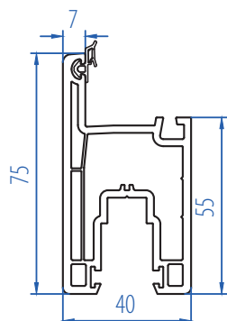
Sliding Sash 2105-1102
