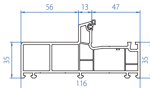
Frame with Grill & Mesh 2101-1102
