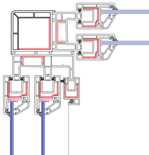
90° Corner Coupling 2108-3101
