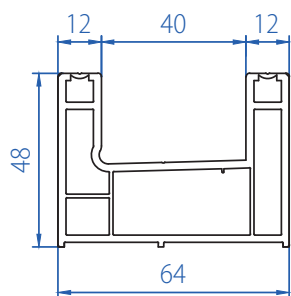
2T Sliding Frame 3104-3101
