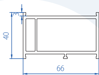
Coupling/ Extension Profile 2108-3106
