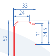
Sliding Door sash (Primary) 2.0mm:9205-2003
