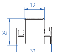
Fly Mesh Sash (Small) Mullion 50502-11037
