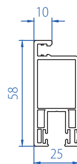
Fly Mesh Sash (Big) 2105-3105
