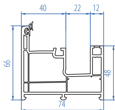
Monorail Sliding Frame 2104-1104
