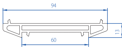
Casement-Sliding Profile Middle Coupler (PRIMA) 50502-11040
