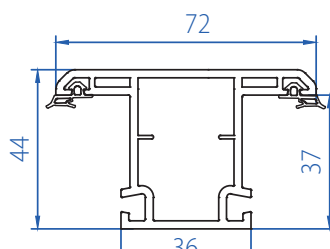
Sliding Mullion 3102-1104
