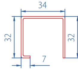
Super Sash Reinforcement 2mm:9305-2002
