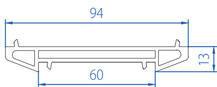
Casement-Sliding Profile Middle Coupler (PRIMA) 50502-11040
