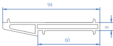
Casement-Sliding Profile Coupler (PRIMA) 50502-11039
