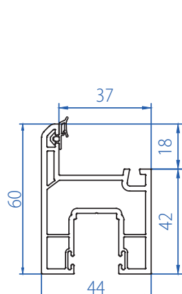
Sliding Window Sash (Non-Euro groove) 3105-1101
