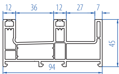
Sliding Frame with Mesh 2104-3103
