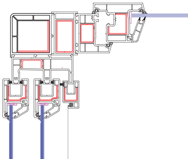
Extension Profile 2108-3106
