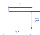
Outward Door Sash 2mm:9203-2002
