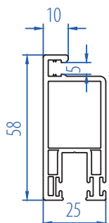
Fly Mesh Sash (Big) 2105-3105
