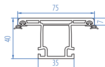
Sliding Mullion 2102-1104
