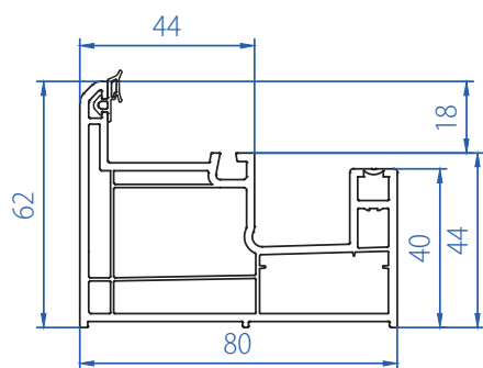
Monorail Sliding Frame 3104-1104
