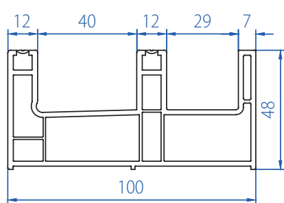
Sliding Frame with Mesh 3104-3103
