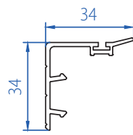
Sash Cover 40502-13100
