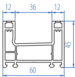
2T Sliding Frame 2104-3101
