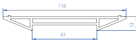
Casement-Sliding Profile Middle Coupler (SUPRA) 50502-11064
