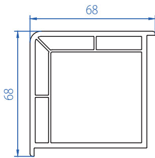
90° Corner Coupling 2108-3101
