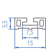
lap strip 41064-40400G
