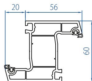
Z-Mullion 2102-1102
