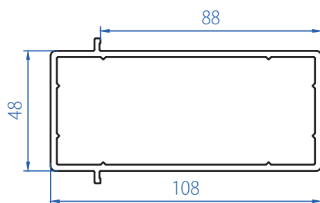
Large Coupling Profile 6108 - 3101
