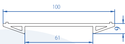
Casement-Sliding Profile Coupler (SUPRA) 50502-11063
