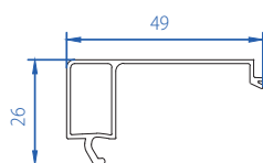
Fixed Louver Clip (PRIMA) 50502-11038
