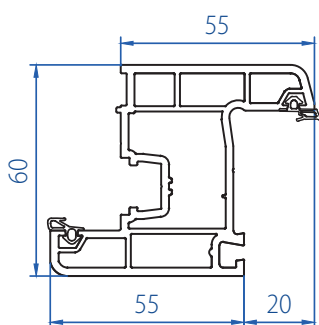
Inward Window Sash 2103-1103
