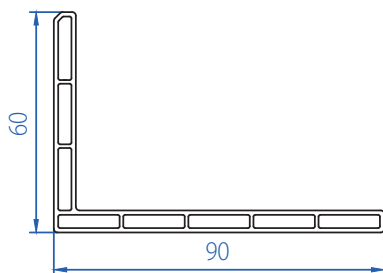
Architrave Profile 2108-3102
