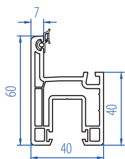
Sliding Window Sash (Non-Euro groove) 2105-1101
