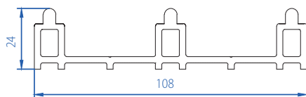
3-Track Low Threshold (PRIMA) 50502-11047
