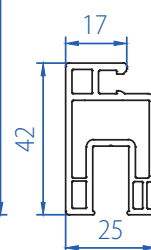
Fly Mesh Sash (Small) 2105-3104
