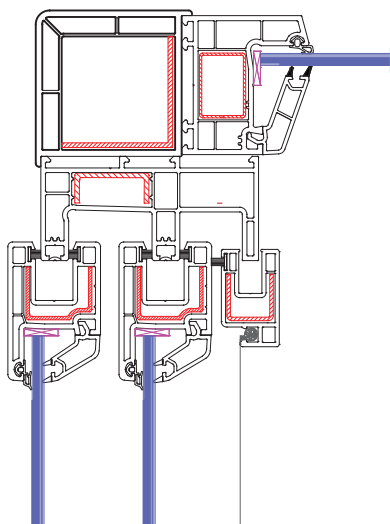
90° Corner Coupling 2108-3101
