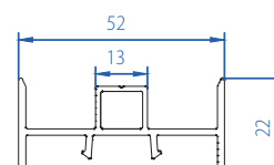
Inline sash adaptor (SUPRA) 50502-11065
