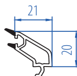
Sliding Single Glazing Bead (5-6mm) 2107-4101
