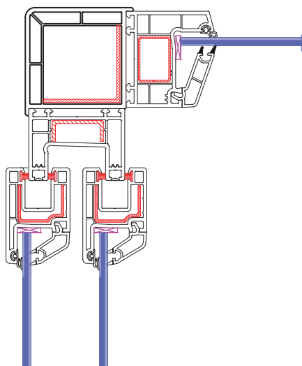
90° Corner Coupling 2108-3101
