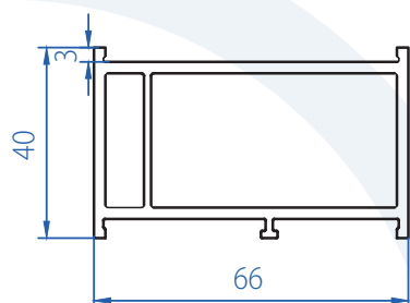
Coupling/ Extension Profile 2108-3106
