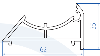
Bay Pole Adaptor 2108-3104
